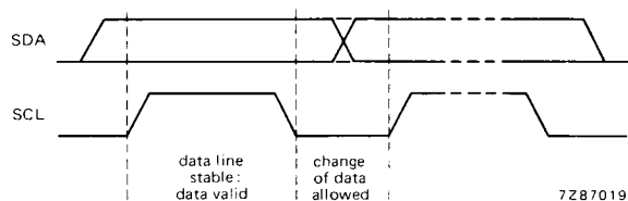
Fig.3 Bit transfer.
