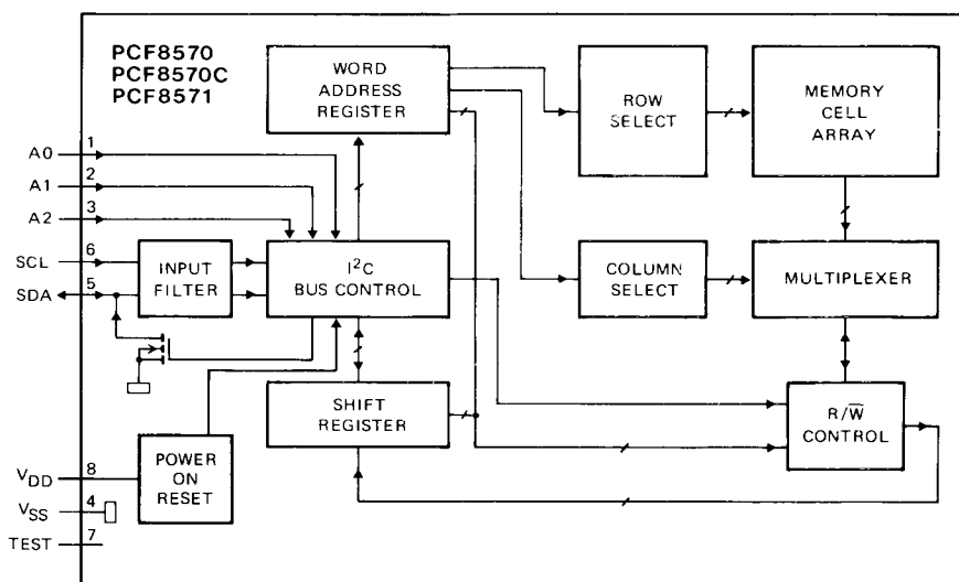
Fig.1 Block diagram.
